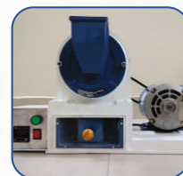
Shiner Lab Polisher
